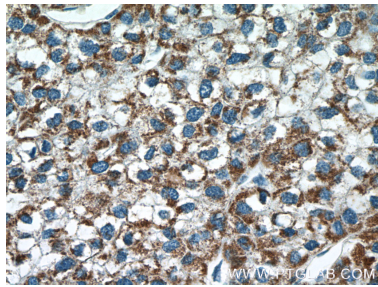
Immunohistochemical analysis of paraffin-embedded human liver cancer tissue slide using 21066-1-AP (MLKL antibody) at dilution of 1:200 (under 40x lens).
